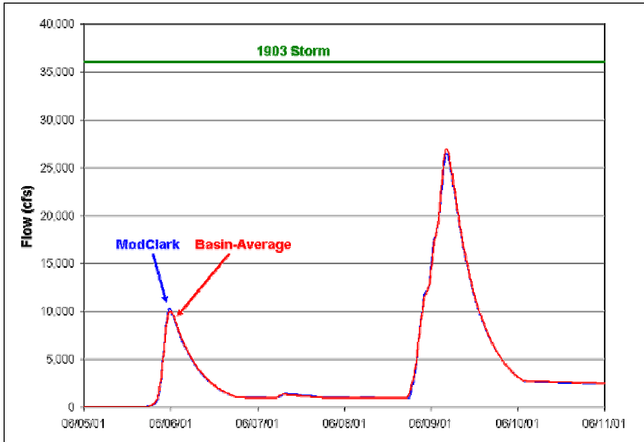
Figure 5: Comparison of modeling results for ModClark and basin-average rainfall input for Tropical Storm Allison-like event to 1903 event.
