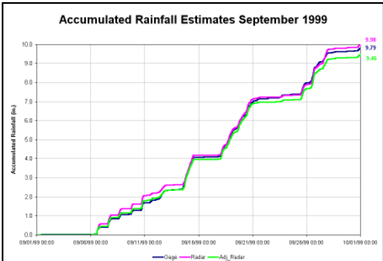
Figure 6: Average accumulated 15-minute rainfall estimates for September 1999
