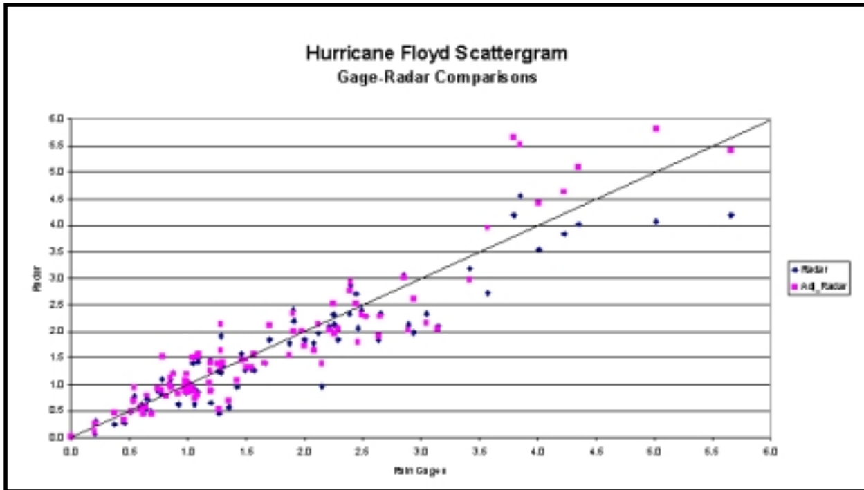
Figure 10: Scatter plot of gage, radar, and gage-adjusted radar-rainfall estimates for Hurricane Floyd
