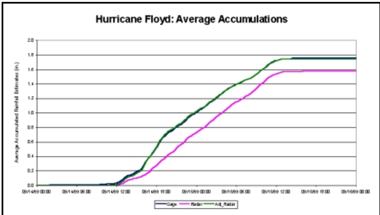
Figure 9: Average rainfall accumulations for Hurricane Floyd
