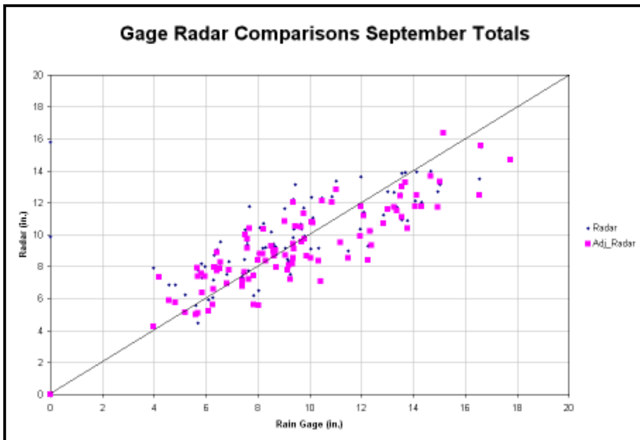
Figure 7: Scatter plot of individual gage vs. radar-rainfall estimates of monthly totals for September 1999
