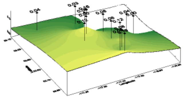
Figure 5: Rainfall contours derived using Kriging (Values are rain gage measurements in inches.)
