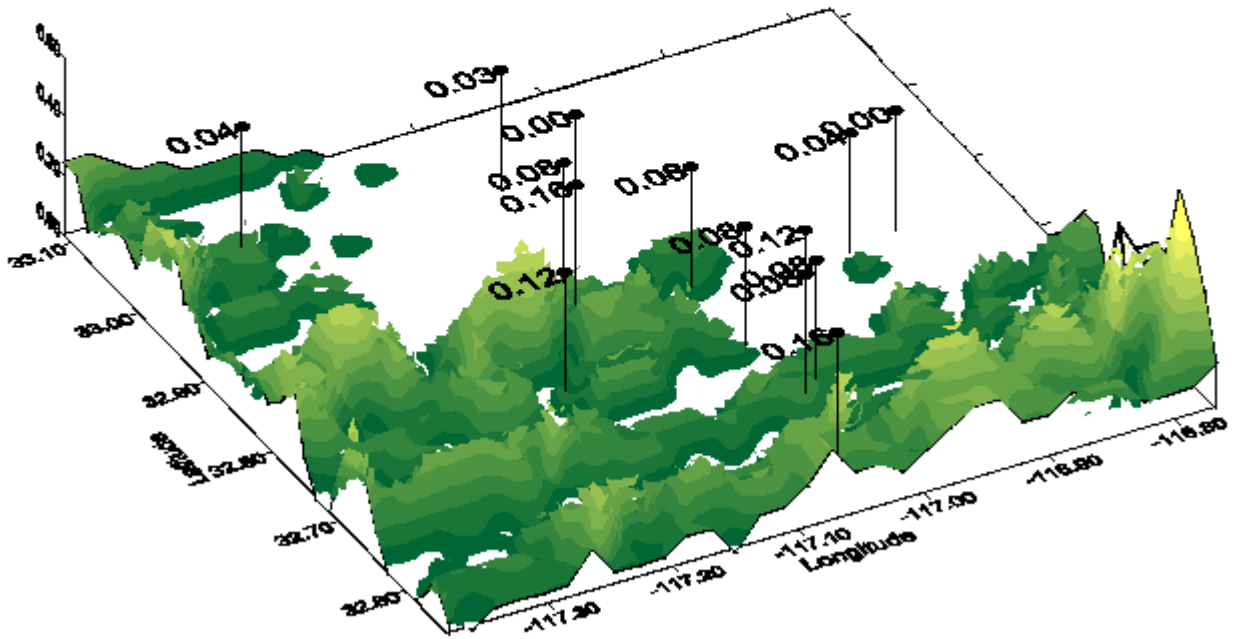
Figure 6: Rainfall contours derived from radar (Values are rain gage measurements in inches.)
