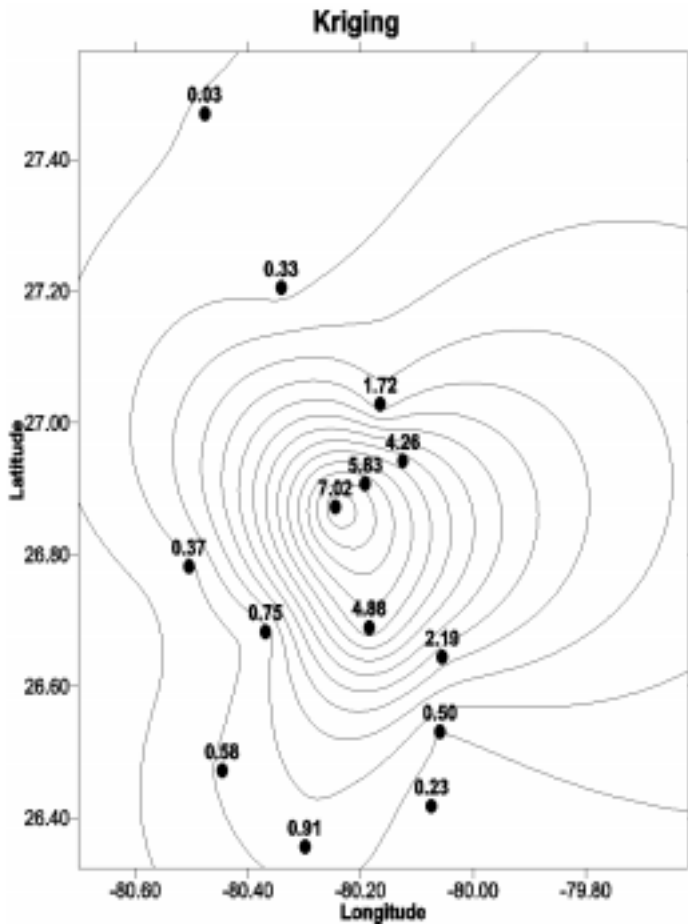
Figure 2: Rainfall contours derived from Kriging (Values are rain gage measurements in inches.)
