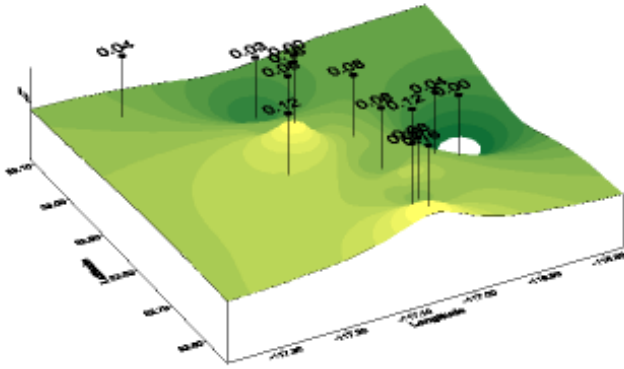
Rainfall Distribution Derived from Inverse Distance Squared
