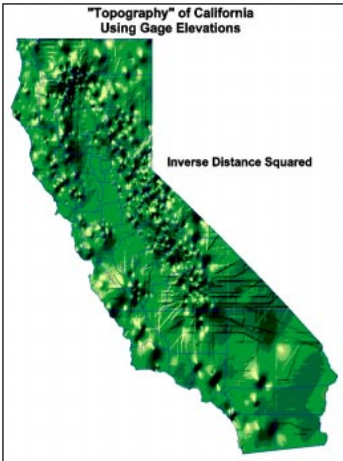
Figure 9: Topography of California derived inverse distance squared weighting
