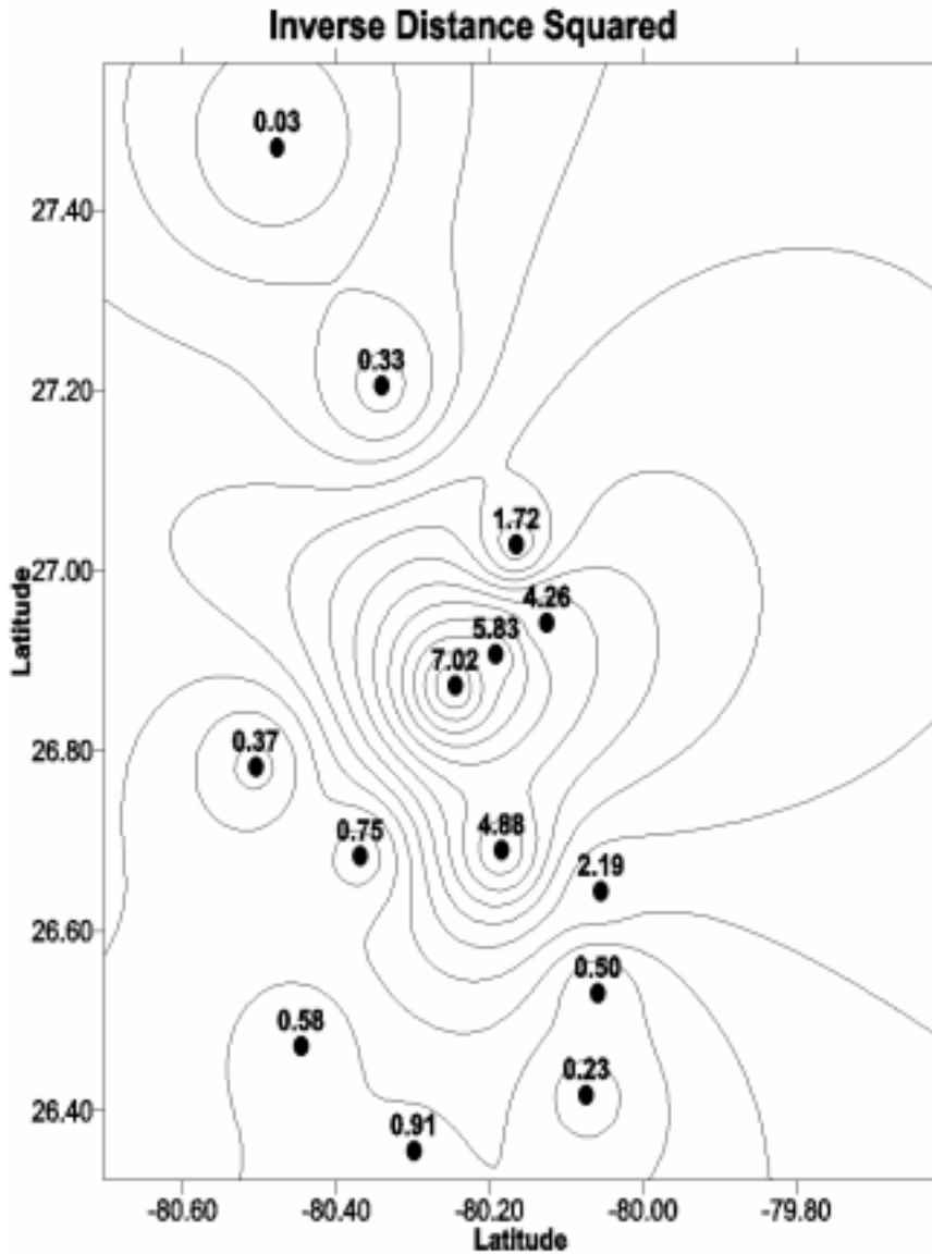
Figure 1: Rainfall contours derived from inverse distance squared weighting (Values are rain gage measurements in inches.)
