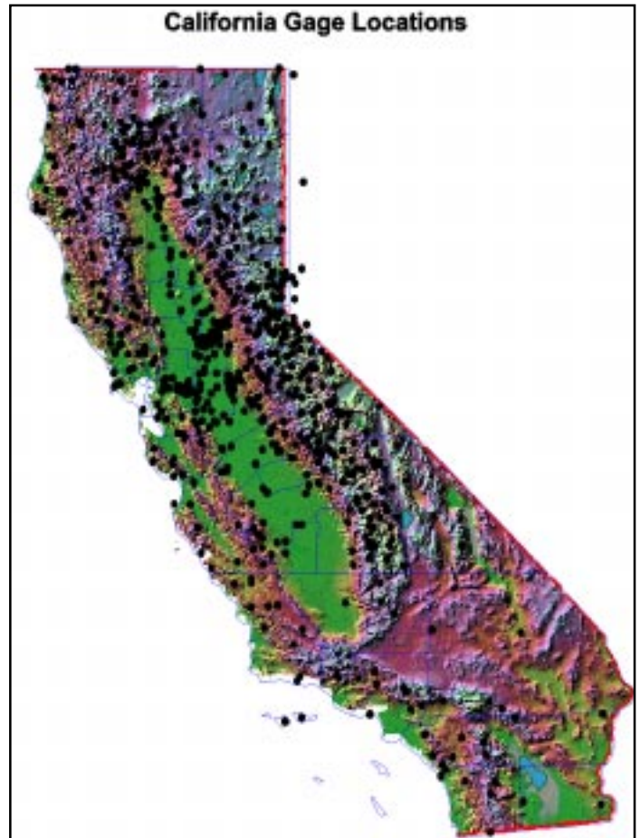
Figure 8: California gage locations
