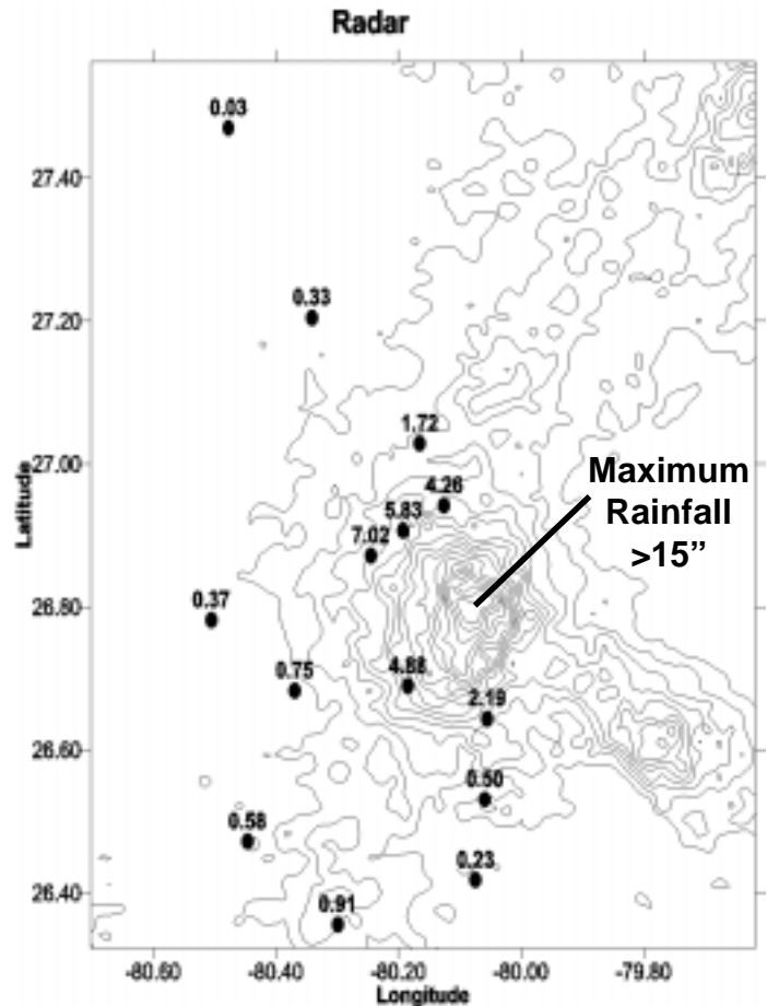
Figure 3: Radar derived rainfall contours (Values are rain gage measurements in inches.)
