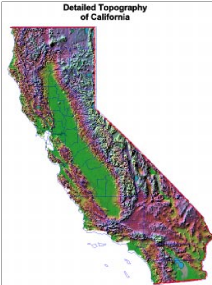
Figure 7: Detailed topography of California
