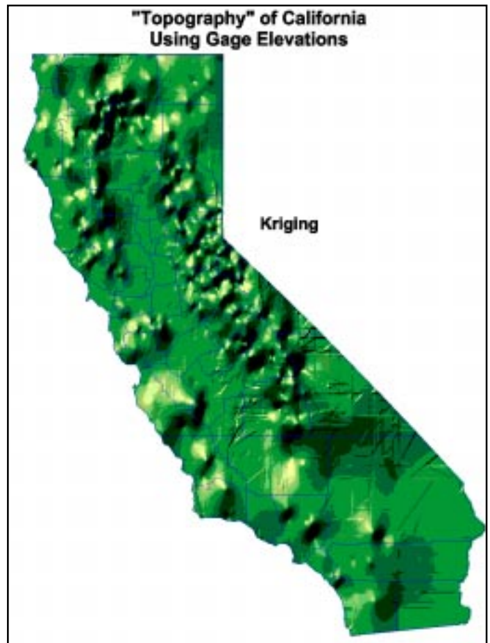
Figure 10: Topography of California derived from Kriging
